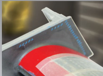
HVMC - High Velocity Masking Compound (blue) and 170-10s Red Plasma Spray Masking Tape
