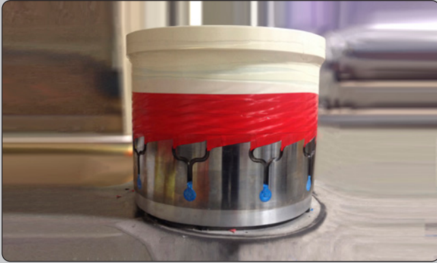
A part masked with 170-10s Red Masking Tape, and High Velocity Masking Compound (Blue) is ready for inspection prior to receiving grit blast.
