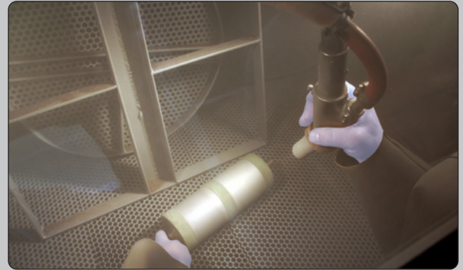
Manual application of grit blast using a handheld nozzle.
