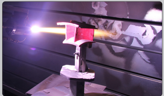
A plasma spray coating is applied to a turbine blade component masked with 170-10S Red Masking Tape.
