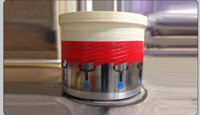
Masking with 170-10s Red Masking Tape, and High Velocity Masking Compound (Blue) which is being used to plug holes.
